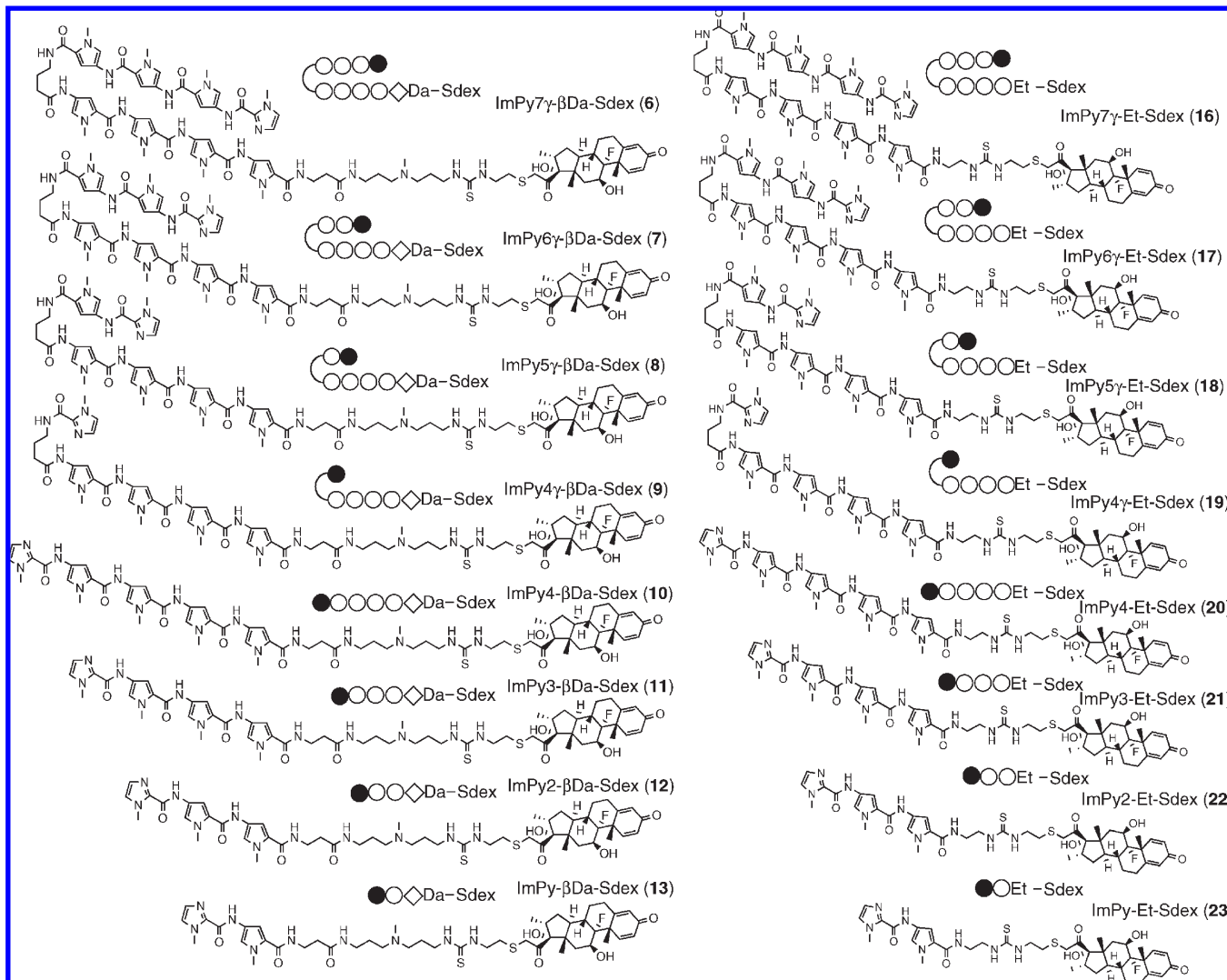
Figure 2. Structures of Py-Im polyamide–Sdex conjugates with \beta Da and Et linkers.
