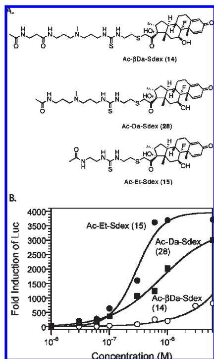
Figure 4. Measurement of the cellular permeability of the linkers: (A) structures of linker–Sdex conjugates; (B) dose-dependent Luc activities induced by Ac-βDa-Sdex (○), Ac-Da-Sdex (■), and Ac-Et-Sdex (●).
