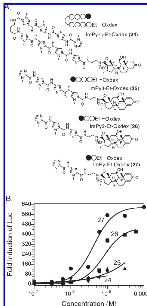
Figure 5. Measurement of the cell permeability of Py-Im polyamide–Oxdex conjugates: (A) structures of Py-Im polyamide–Oxdex conjugates with the Et linker; (B) dose dependent Luc activities induced by Py-Im polyamide–Et–Oxdex conjugates in HeLa cells (●, ImPy-Et-Oxdex; ■, ImPy2-Et-Oxdex; ▲, ImPy3-Et-Oxdex; ▼, ImPy7γ-Et-Oxdex).
